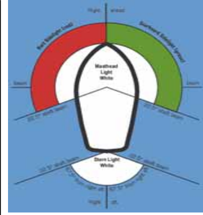
Serial N/O 554 LED side lights Vertical mount
